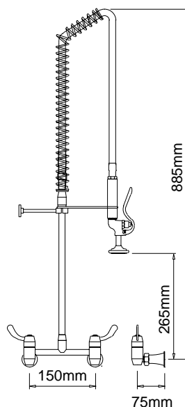
Exposed Mixer Assembly / Spring Return Product Code: FWS 031 With pot filler: FWS 131 *215mm width or adjustable centres are also available.
