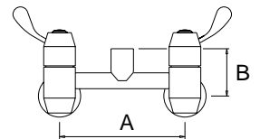
WALL EXPOSED MIXER FS 022: A 150mm B 90mm *215mm width or adjustable centres are also available.
