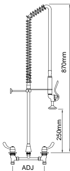
Concealed Mixer Assembly / Spring Return Product Code: FHS 021 With pot filler: FHS 121
