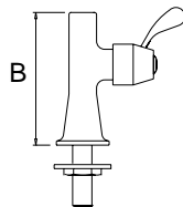
HOB PRE MIXER FS 011: B: 130mm
