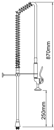
Riser Assembly / Spring Return Product Code: FHS 001 With pot filler: FHS 101
