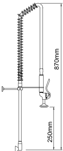
Riser Assembly / Spring Return Product Code: FWS 001 With pot filler: FWS 101
