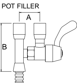
FS 063: A 45mm B 120mm
