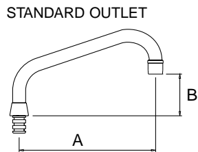
FS 180: 180mm 70mm FS 181: 230mm 95mm FS 182: 300mm 110mm With aerator
