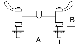
HOB EXPOSED MIXER FS 012: A: 150mm B: 290mm *215mm width or adjustable centres are also available.
