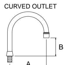
FS 184: 150mm 100mm FS 185: 200mm 90mm With aerator
