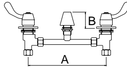
HOB CONCEALED MIXER FS 013: A: 140 - 230mm B: 40mm
