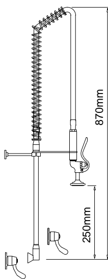
Concealed Mixer Assembly / Spring Return Product Code: FWS 021 With pot filler: FWS 121
