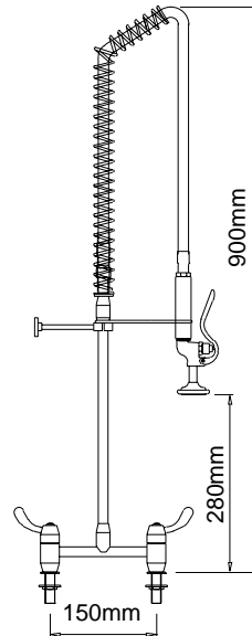
Exposed Mixer Assembly / Spring Return Product Code: FHS 031 With pot filler: FHS 131 *215mm width or adjustable centres are also available.
