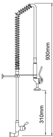
Pre-Mixer Assembly / Swivel Arm Product Code: FWS 011 With pot filler: FWS 111
