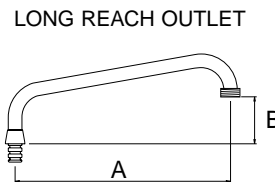
FS 188: 150mm 50mm FS 187: 300mm 80mm With 1/2" BSP thread
