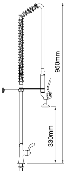
Pre-Mixer Assembly / Swivel Arm Product Code: FHS 011 With pot filler: FHS 111
