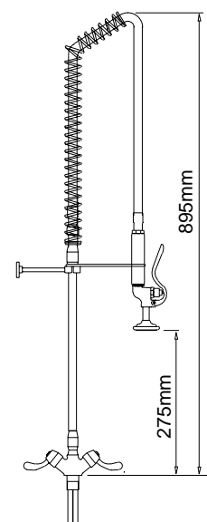
Dual Mixer Assembly / Spring Return Product Code: FHS 041 With pot filler: FHS 141
