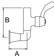
WALL PRE MIXER FS 021: A 80mm B 100mm
